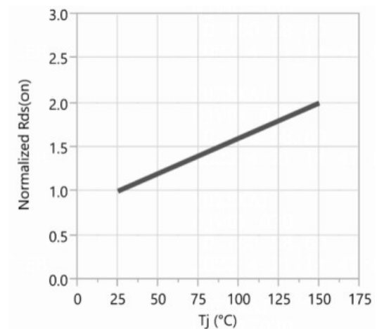
Figure 4. Normalized On-resistance
