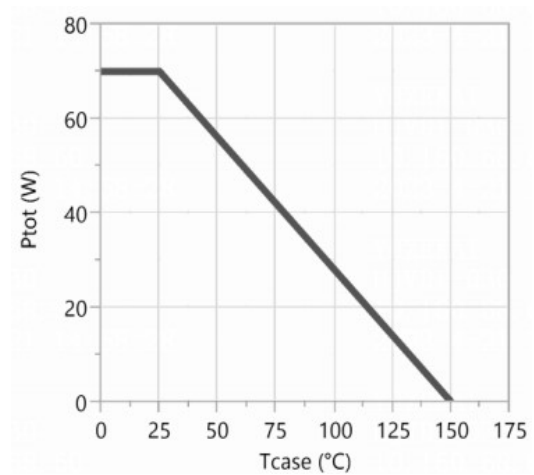
Figure 10. Power Dissipation
