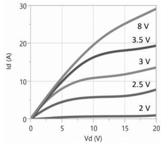
Figure 2. Typical Output Characteristics T_J=150^{\circ}C
