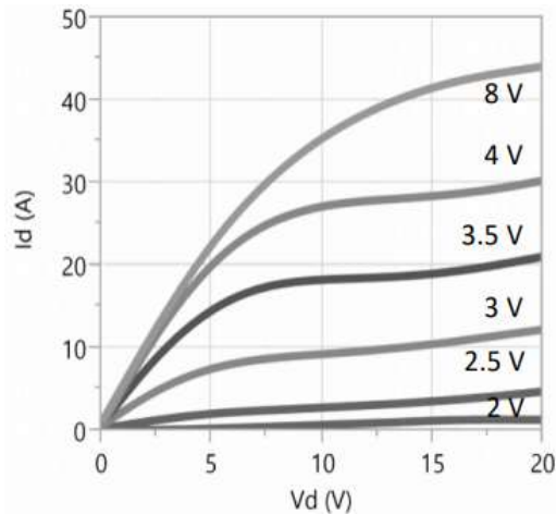
Figure 1. Typical Output Characteristics T_J=25^{\circ}C
