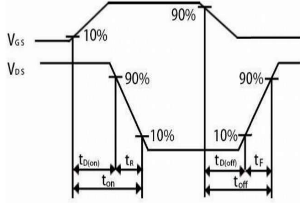
Figure 16. Switching Time Waveform
