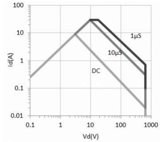
Figure 14. Safe operating Area T_C=80^{\circ}C (calculated based on thermal limits)
