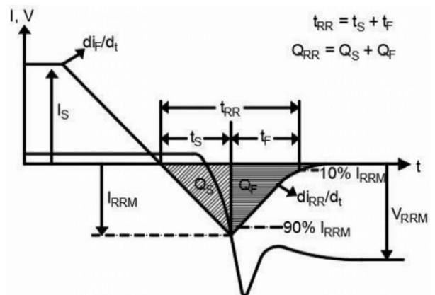
Figure 20. Diode Recovery Waveform
