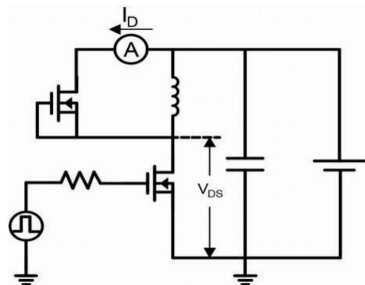
Figure 19. Diode Characteristic Test Circuit
