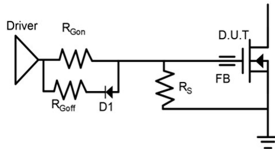
Recommended Single Ended Drive Circuit
