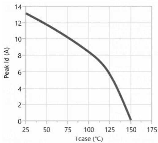
Figure 11. Current Derating
