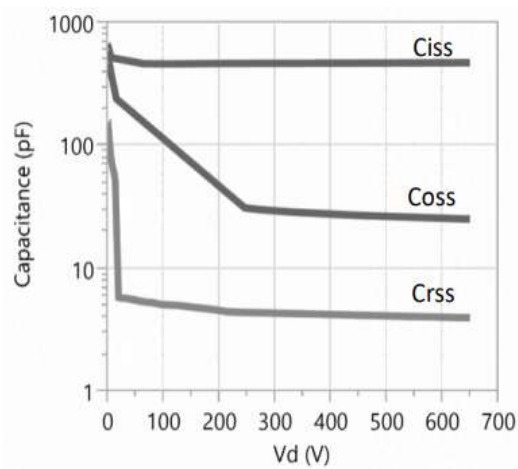
Figure 5. Typical Capacitance
