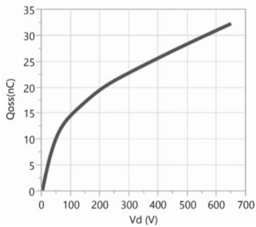
Figure 7. Typical Qoss
