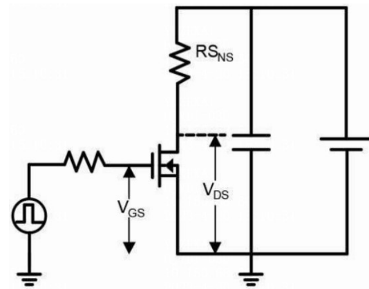
Figure 17. Dynamic R_{DS(on)} Test Circuit
