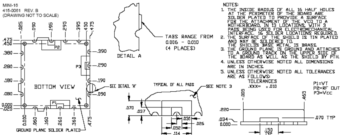
PHYSICAL DIMENSIONS
