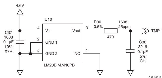
Figure 7.2 Temperature Sensors
