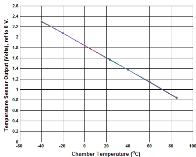
Figure 6.24 Temperature Sensor Output with respect to 0V (GND) against Chamber Temperature for CRS09-01 and CRS09-11
