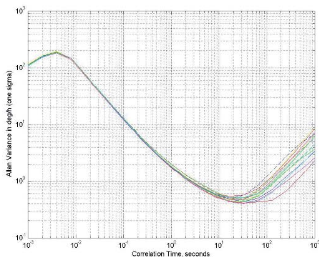
Figure 6.22 Typical Allan Variance Data for CRS09-02 and CRS09-12
