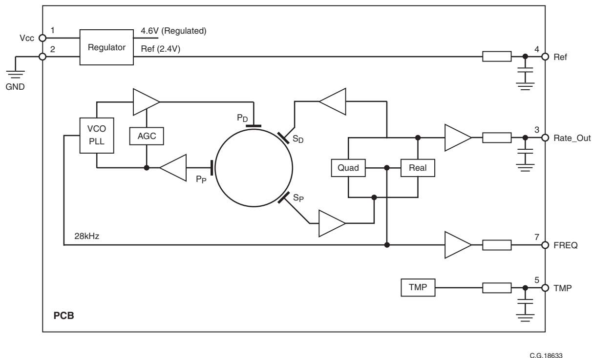
Figure 1.1 CRS09 Functional Block Diagram
