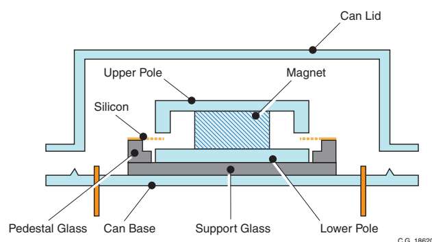
Figure 10.2 MEMS Sensor Head
