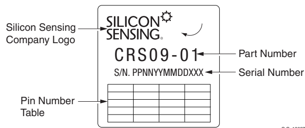
Figure 9.1 Part Marking
