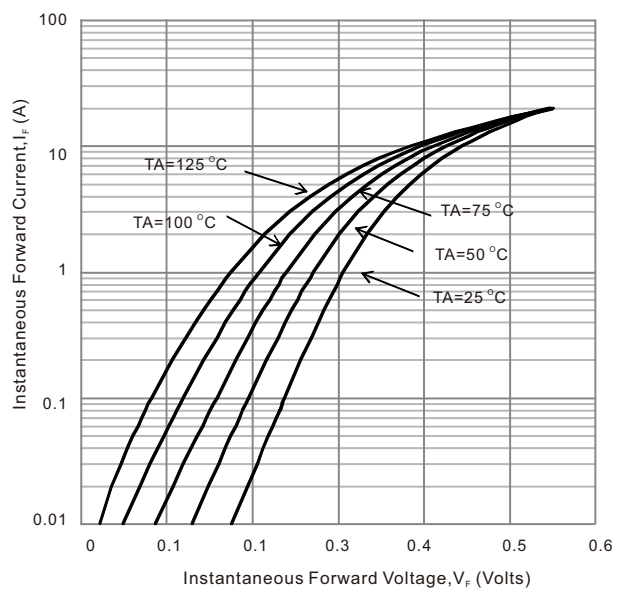
Fig. 2 - Instantaneous Forward Characteristics
