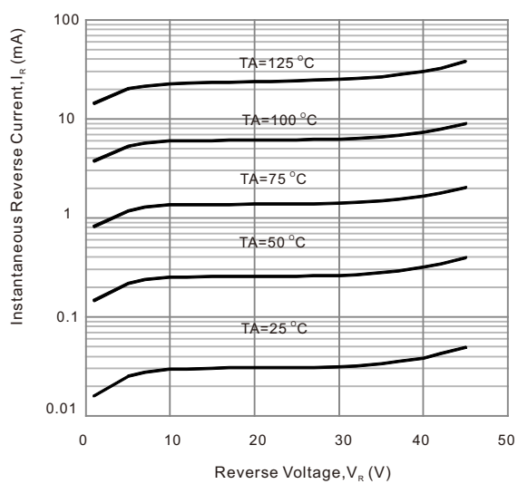
Fig. 3 - Reverse Characteristics
