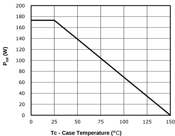
Fig 11: Power Dissipation
