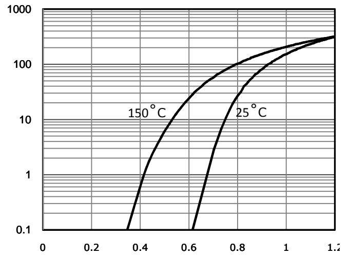
Fig 8: Body-diode Forward Characteristic
