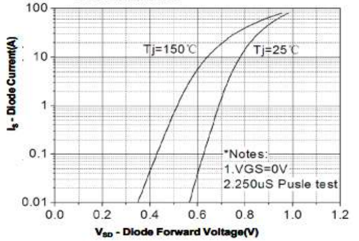
Fig 8: Body-diode Forward Characteristics
