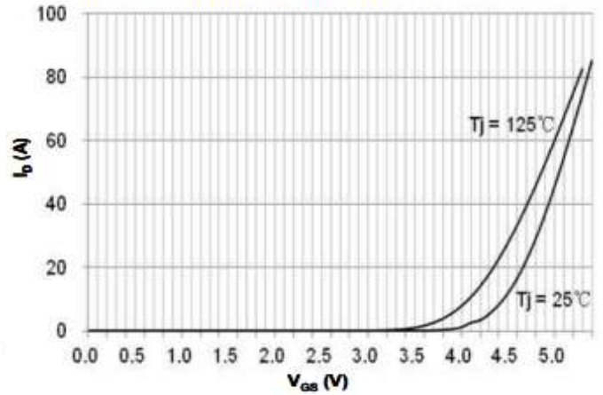
Fig 2: Transfer Characteristics
