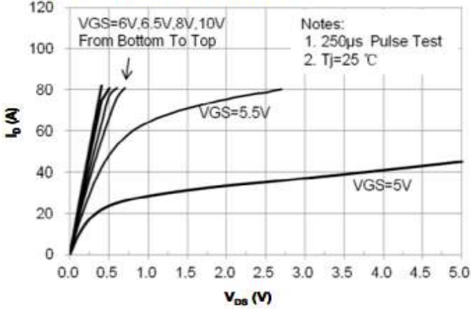
Fig 1: Output Characteristics
