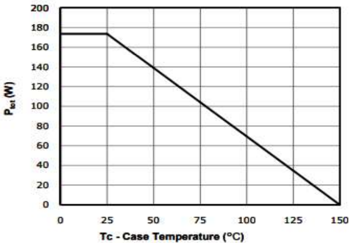
Fig 9: Power Dissipation
