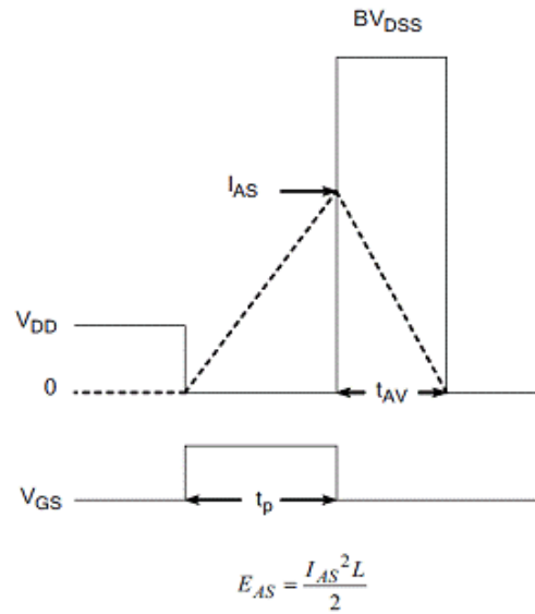
Figure 22. Unclamped Inductive Switching Waveform
