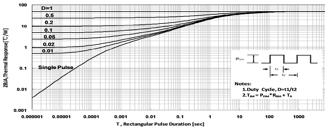
Figure 5 Maximum Effective Thermal Impedance , Junction to Ambient
