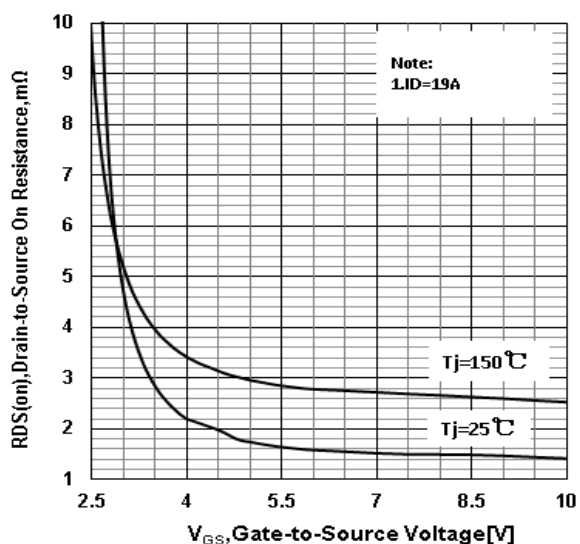
Figure 14 . Drain-to-Source On Resistance vs Gate Voltage
