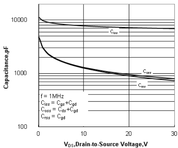
Figure 12. Capacitance Characteristics
