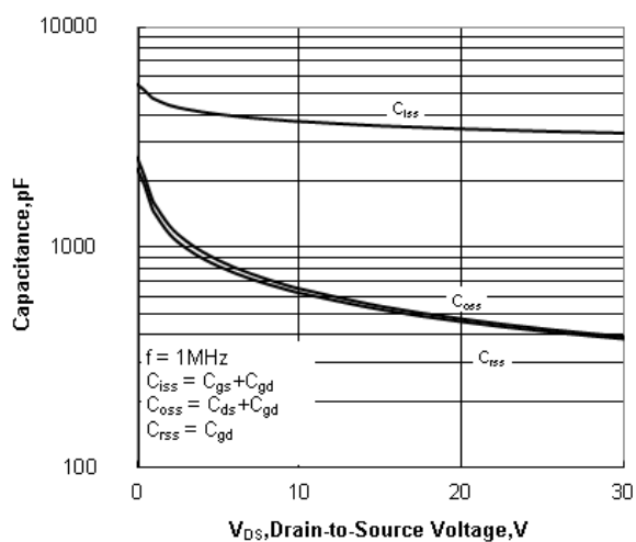
Figure 12. Capacitance Characteristics
