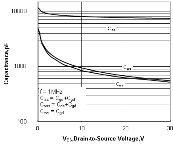
Figure 12. Capacitance Characteristics
