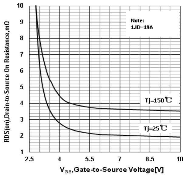
Figure 14 . Drain-to-Source On Resistance vs Gate Voltage
