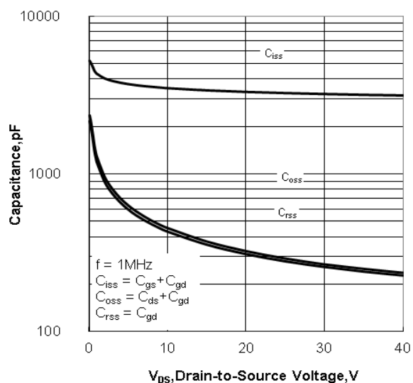
Figure 12. Capacitance Characteristics
