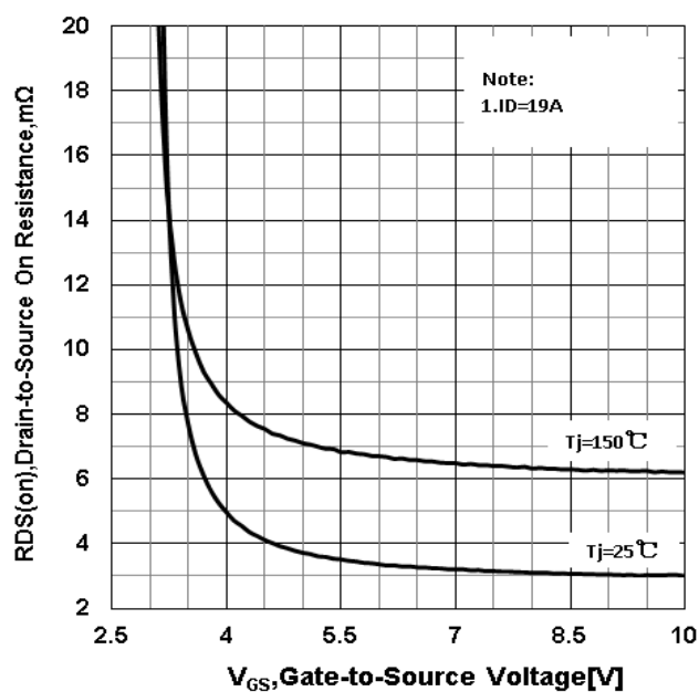
Figure 14 . Drain-to-Source On Resistance vs Gate Voltage
