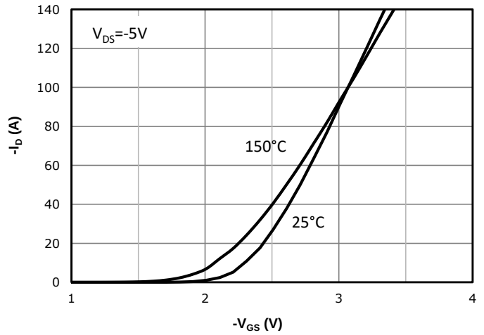
Fig 2: Transfer Characteristics
