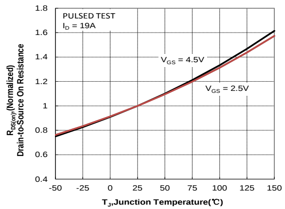
Figure 9. Normalized On Resistance vs Junction Temperature
