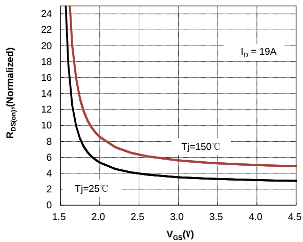
Figure 14. Normalized On Resistance vs VGS
