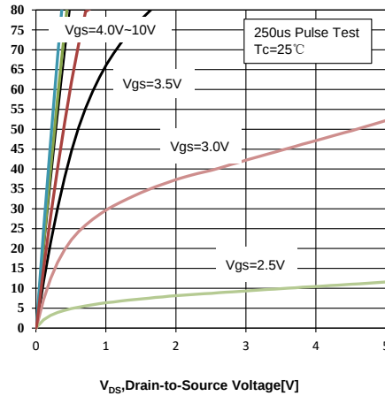
Figure 4. Typical output Characteristics
