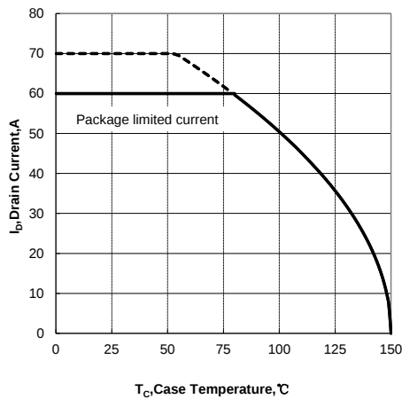
Figure 3. Maximum Continuous Drain Current vs Case Temperature
