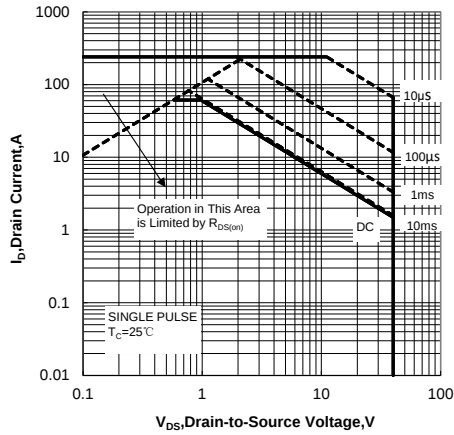
Figure 1. Maximum Safe Operating Area
