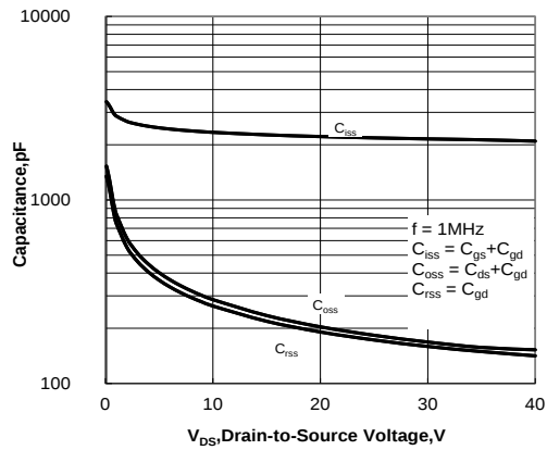
Figure 12. Capacitance Characteristics
