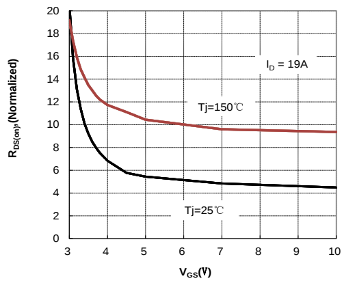
Figure 14. Normalized On Resistance vs V_{GS}
