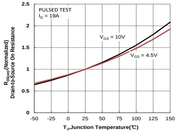
Figure 9. Normalized On Resistance vs Junction Temperature
