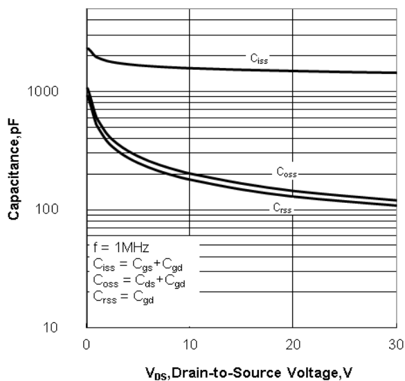
Figure 12. Capacitance Characteristics
