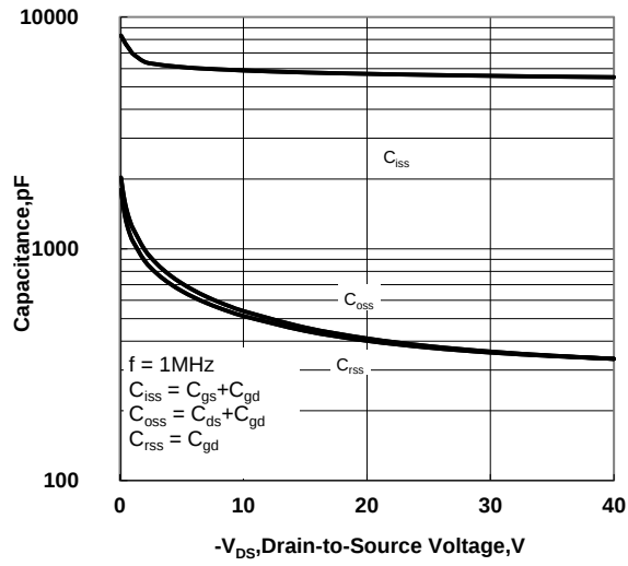
Figure 12. Capacitance Characteristics
