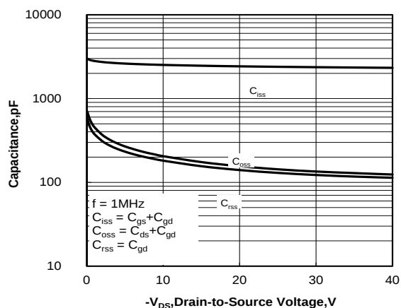
Figure 12. Capacitance Characteristics
