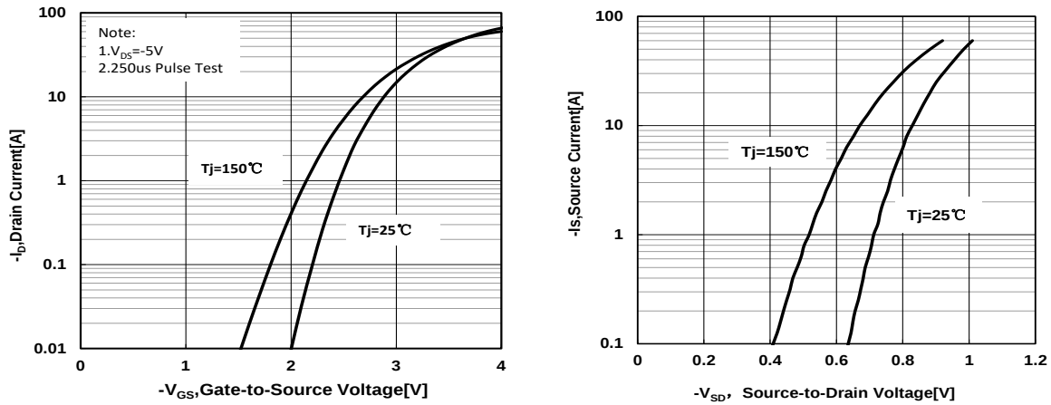
Figure 6 Typical Transfer Characteristics
