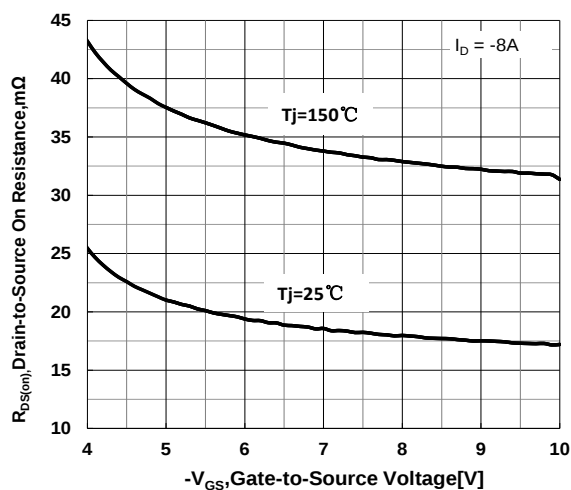
Figure 14 Drain-to-Source On Resistance Gate-to-Source Voltage
