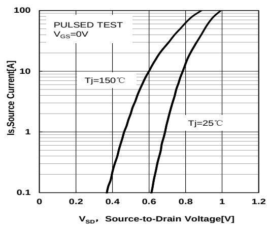
Figure 7 Typical Body Diode Transfer
