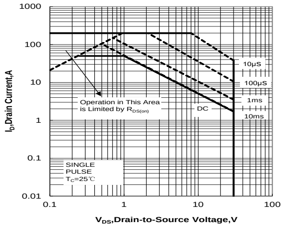
Figure 1 . Maximum Safe Operating
