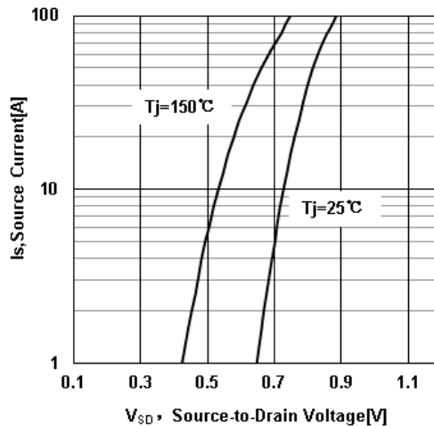
Figure 7 Typical Body Diode Transfer Characteristics
