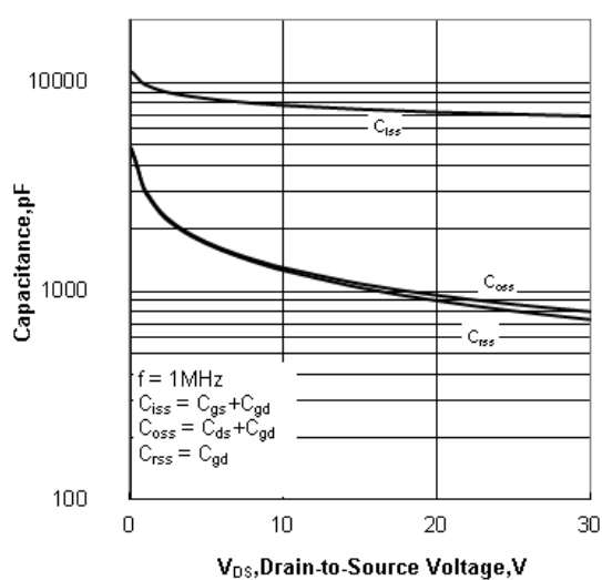
Figure 12. Capacitance Characteristics
