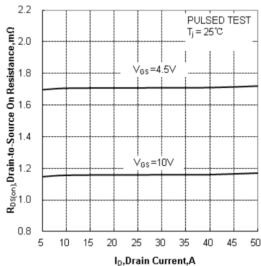
Figure 8. Drain-to-Source On Resistance vs Drain Current
