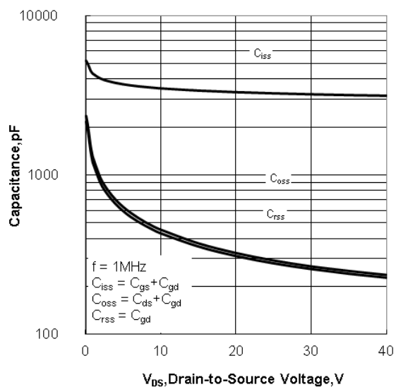
Figure 12. Capacitance Characteristics
