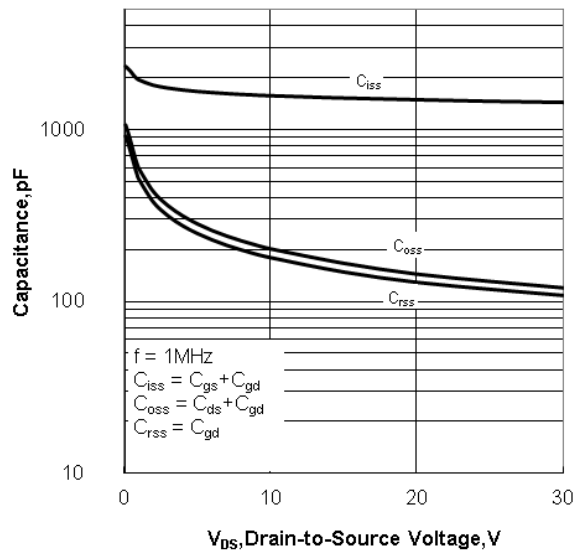
Figure 12. Capacitance Characteristics
