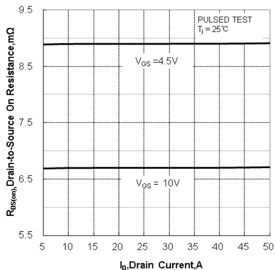
Figure 8. Drain-to-Source On Resistance vs Drain Current
