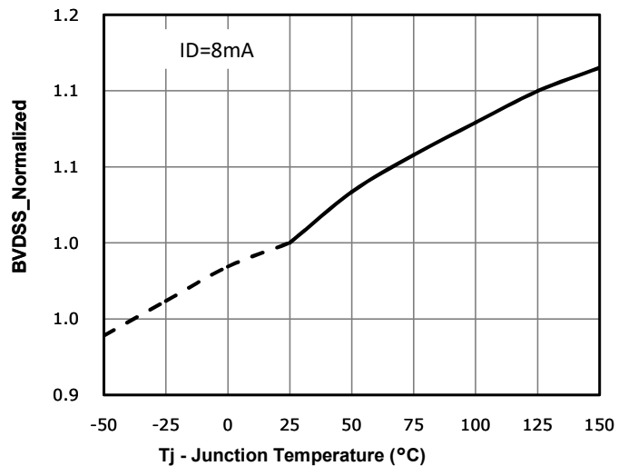
Fig 6: BVDSS vs. Temperature
