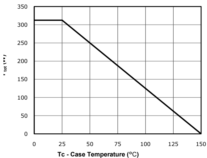
Fig 11: Power Dissipation
