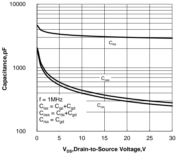
Figure 12. Capacitance Characteristics
