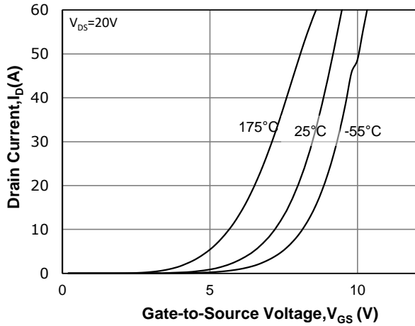
Fig 7: Transfer Characteristics
