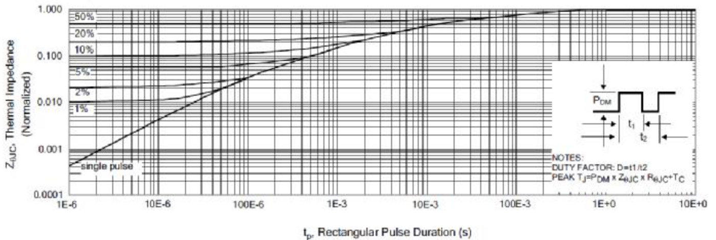
Figure 5 Maximum Effective Thermal Impedance, Junction to Case
