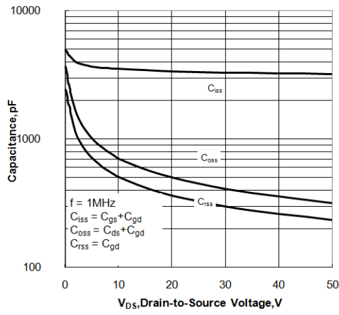
Figure 12. Capacitance Characteristics
