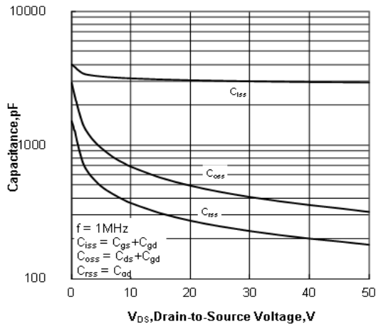
Figure 12. Capacitance Characteristics
