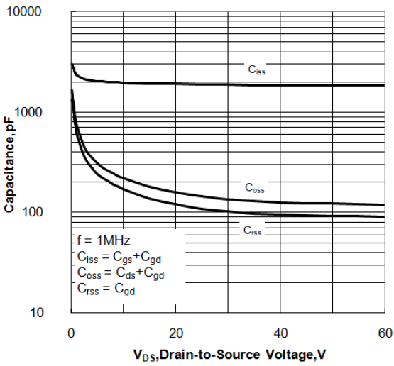
Figure 12. Capacitance Characteristics
