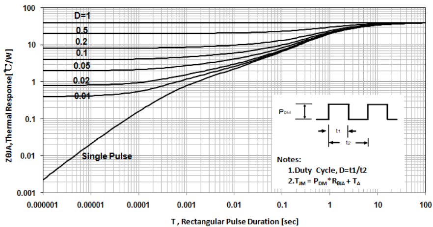
Figure 5 Maximum Effective Thermal Impedance, Junction to Ambient
