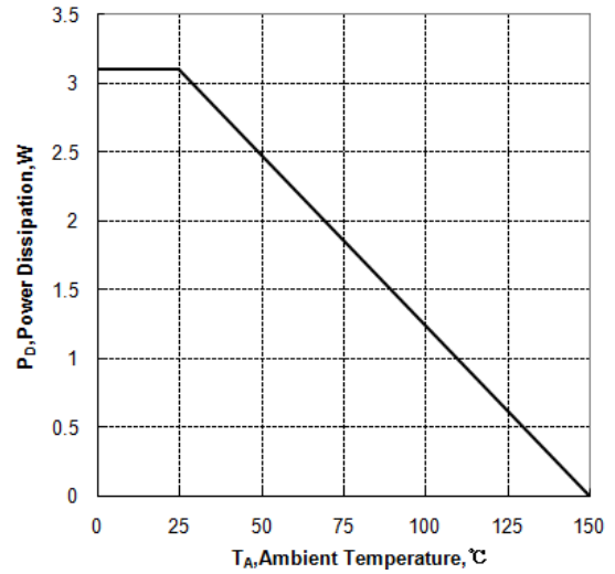
Figure 2. Maximum Power Dissipation vs Ambient Temperature
