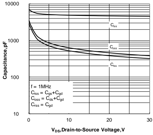
Figure 12. Capacitance Characteristics
