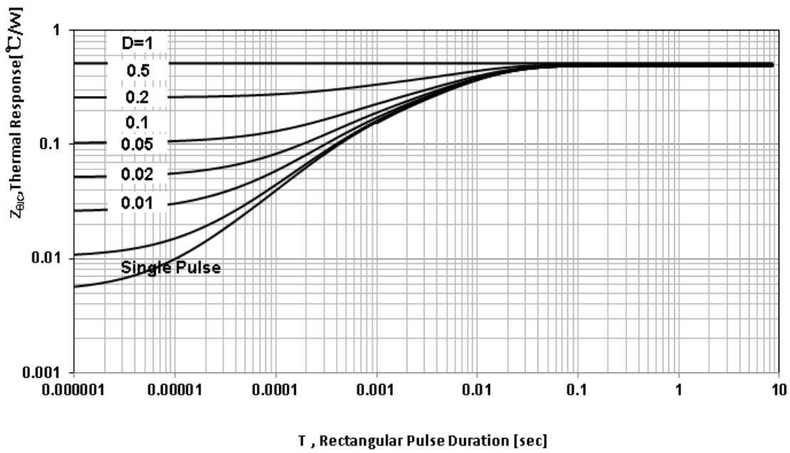
Figure 13 Maximum Effective Transient Thermal Impedance, Junction-to-Case
