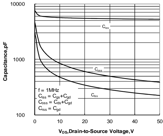
Figure 12. Capacitance Characteristics
