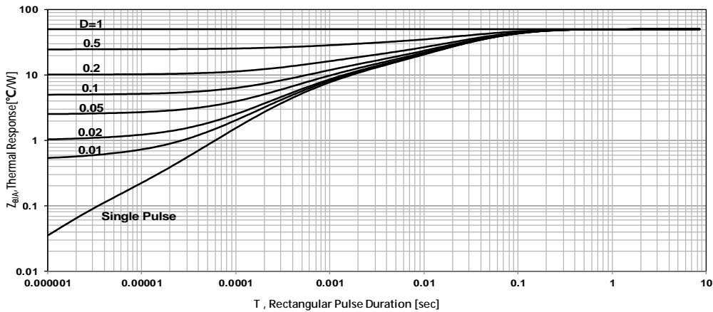
Figure 5 Maximum Effective Thermal Impedance , Junction to Ambient
