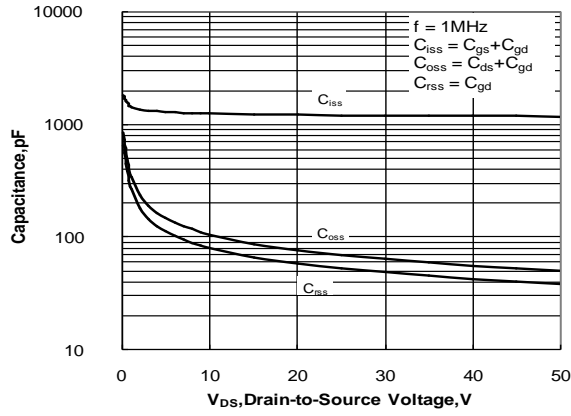
Figure 12. Capacitance Characteristics
