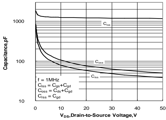
Figure 12. Capacitance Characteristics
