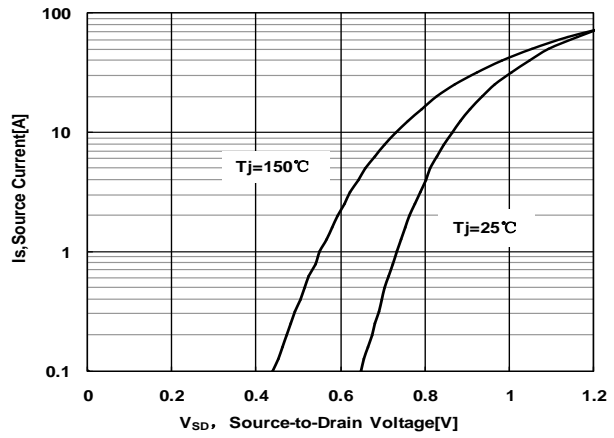
Figure 7 Typical Body Diode Transfer Characteristics
