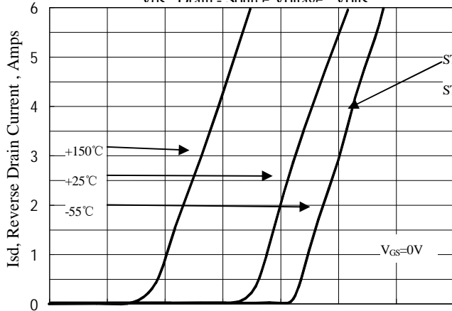
Figure 15 Typical Body Diode Transfer Characteristics
