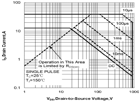
Figure 1 Maximum Forward Bias Safe Operating Area
