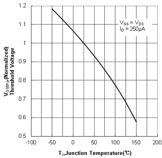
Figure 11 Typical Theshold Voltage vs Junction Temperature
