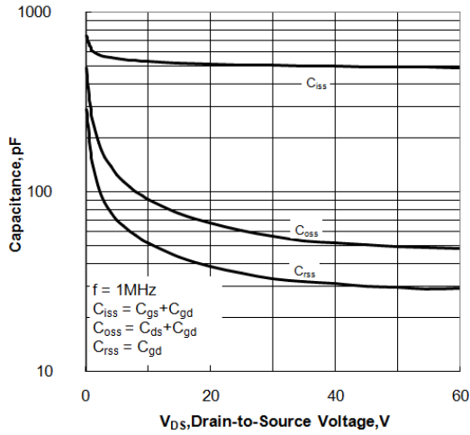
Figure 12. Capacitance Characteristics
