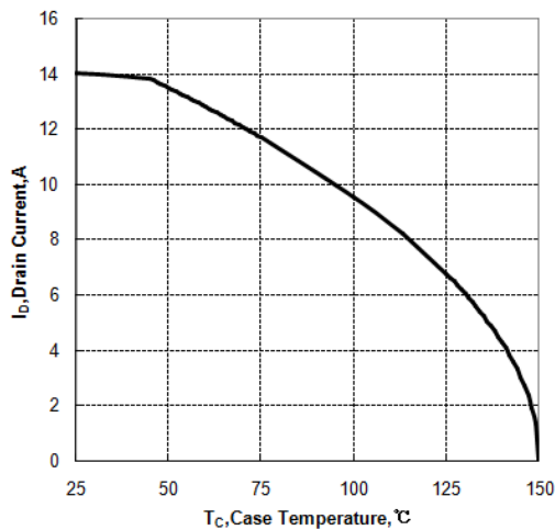
Figure 3. Maximum Continuous Drain Current vs
