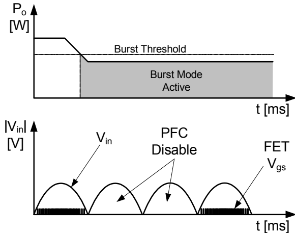
Figure 14. Burst Mode
