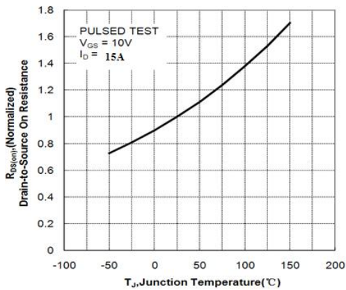
Figure 11. Typical Drain to Source on Resistance vs Junction Temperature
