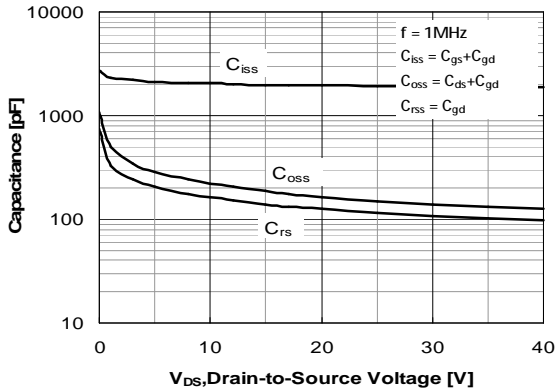
Figure 9. Typical Capacitance vs Drain to Source Voltage
