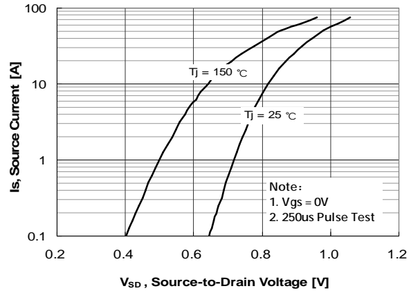
Figure 8. Body Diode Forward Voltage vs Source Current
