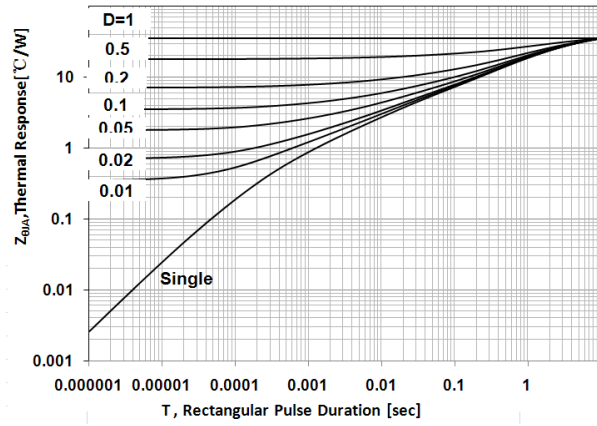
Figure 14 .Maximum Effective Transient Thermal Impedance
