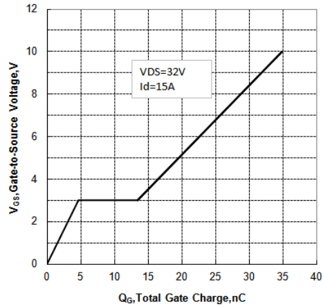
Figure 10. Gate Charge Characteristics
