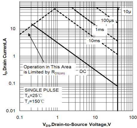
Figure 1. Maximum Safe Operating Area
