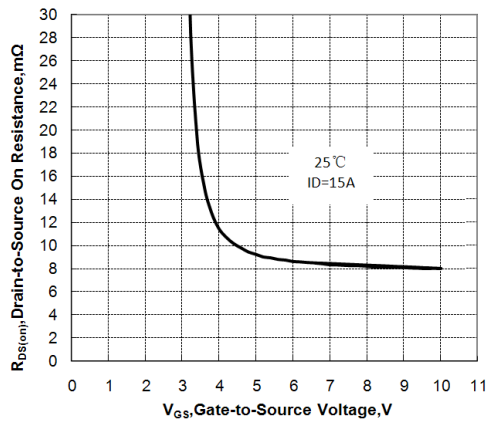
Figure 7. Drain-to-Source On Resistance vs Gate Voltage
