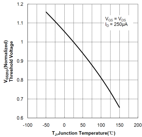
Figure 12. Typical Threshold Voltage vs Junction Temperature
