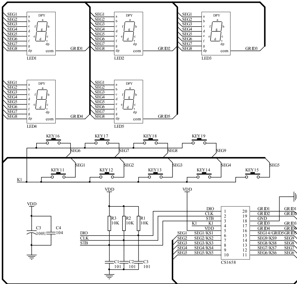
COMMON CATHOD TYPE LED PANEL:
