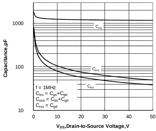
Figure 12. Capacitance Characteristics
