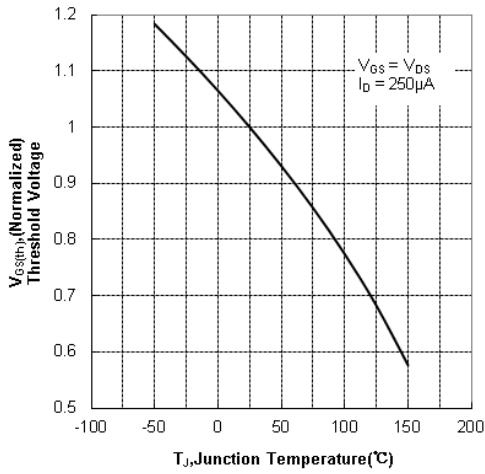
Figure 11 Typical Theshold Voltage vs Junction Temperature
