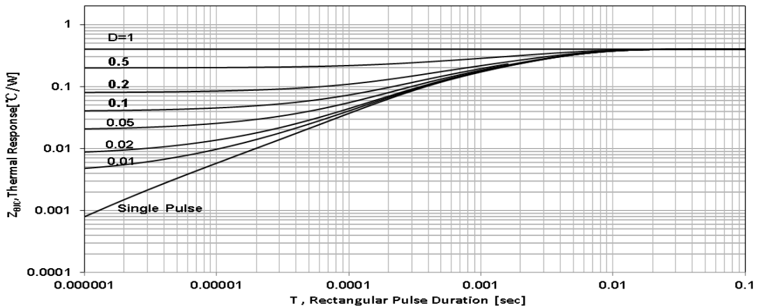
Figure5. Maximum Effective Transient Thermal Impedance, Junction-to-Case
