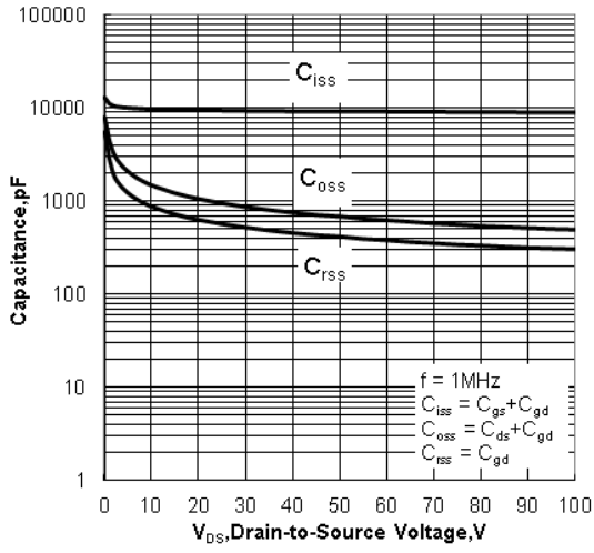
Figure12. Capacitance Characteristics
