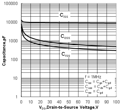
Figure12. Capacitance Characteristics
