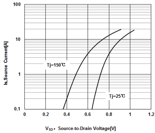
Figure 6 Typical Body Diode Transfer Characteristics
