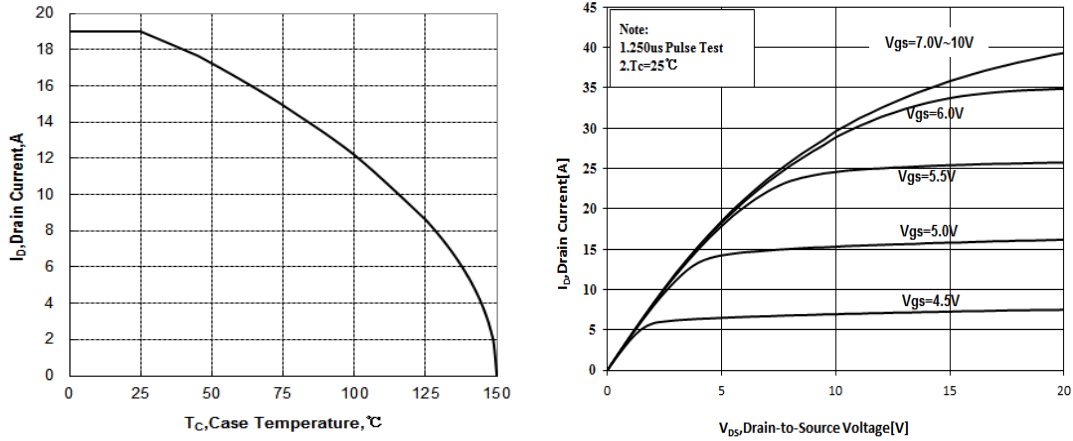
Figure 2 Maximum Continuous Drain Current vs Case Temperature
