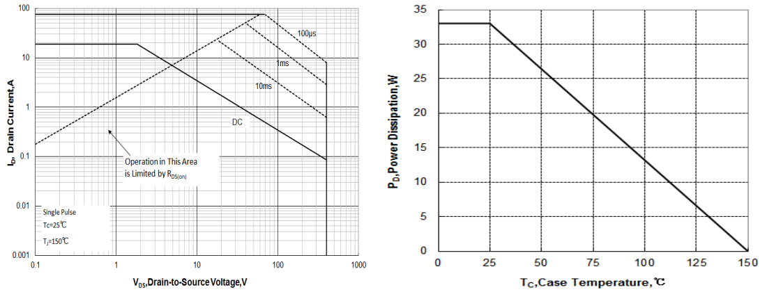
Figure 1 Maximum Power dissipation vs Case Temperature
