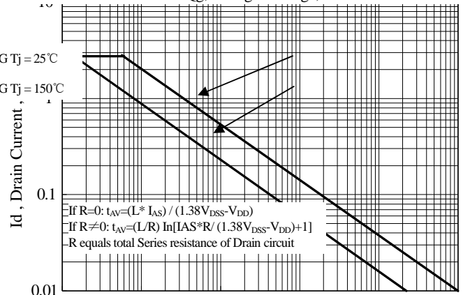
Figure 16 Unclamped Inductive Switching Capability
