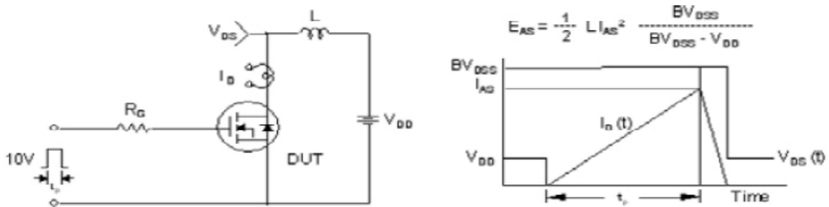
Unclamped Inductive Switching Test Circuit and Waveform
