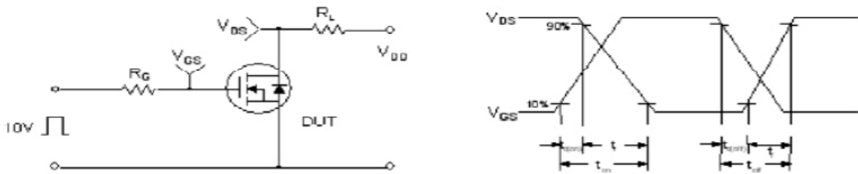
Resistive Switching Test Circuit and Waveform
