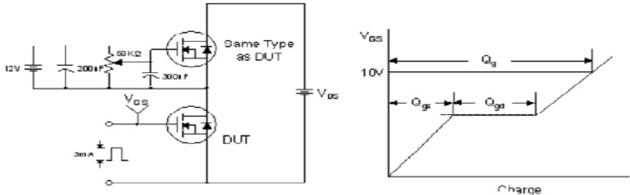
Gate Charge Test Circuit and Waveform
