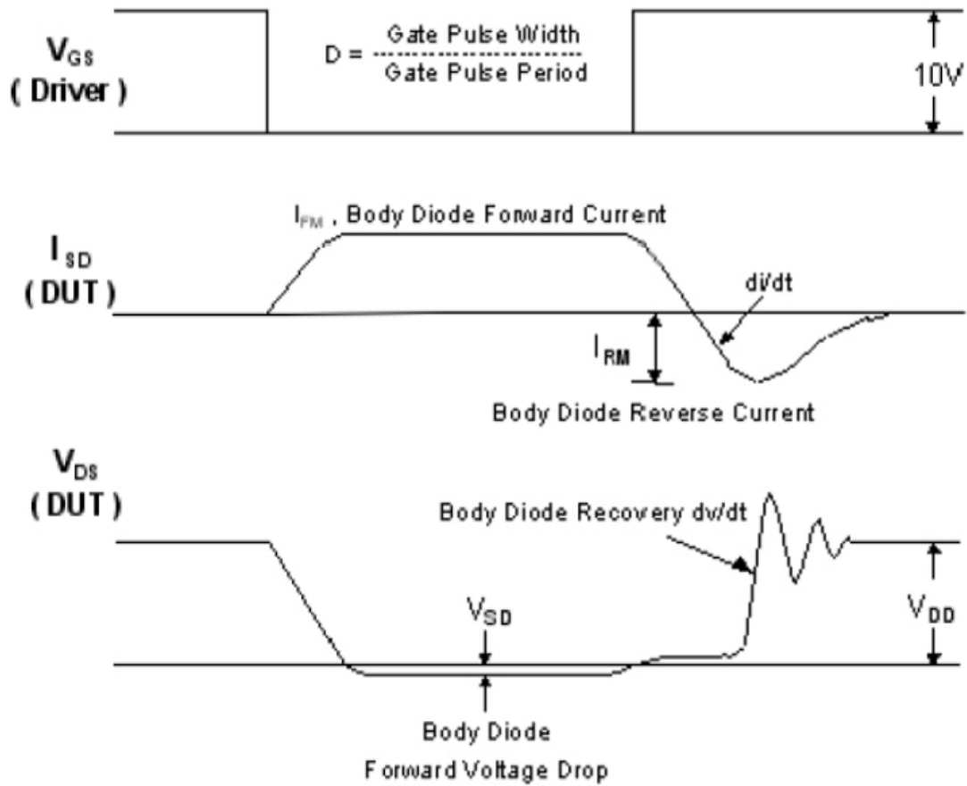
Diode Reverse Recovery Test Circuit and Waveform
